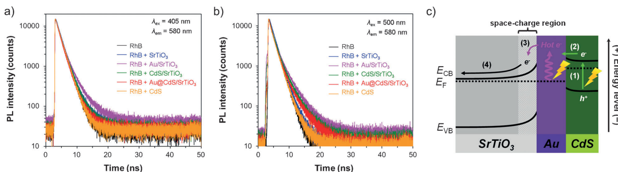
Figure 3. Time-resolved PL spectra of a RhB solution (1 μM) in the presence of the indicated sample with a) excitation at 405 nm and b) excitation at 500 nm, where the emission wavelength is 580 nm. c) Schematic energy band diagram of Au@CdS/SrTiO 3 , showing the proposed electron-transfer processes across the three components responsible for H 2 production. The numbered arrows indicate the following individual electron-transfer steps: 1) Excitation of electrons in the CdS shell, 2) electron injection from the CB of the CdS shell into the Fermi level of the Au core, 3) plasmon-induced hot electron injection from the Au core into the CB of SrTiO 3 , and 4) migration of the hot electrons to active sites at the surface of SrTiO 3 .
